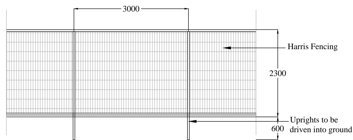
TREE PROTECTION FENCE ELEVATION 1:50
